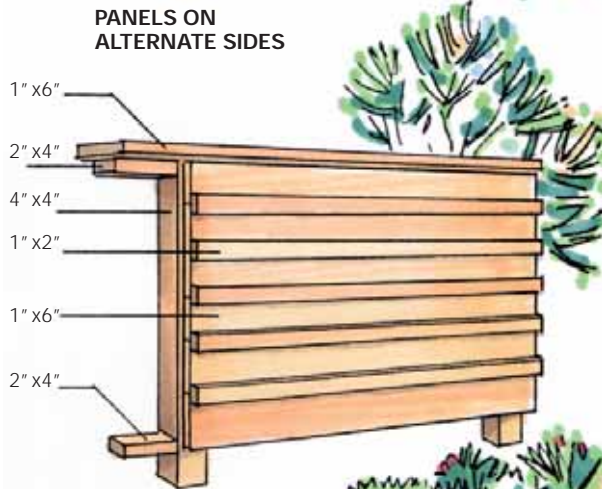
HORIZONTAL BOARD-AND-BATTEN
